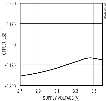
MAX1099 OFFSET vs. SUPPLY VOLTAGE
