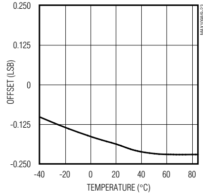
MAX1098 OFFSET vs. TEMPERATURE
