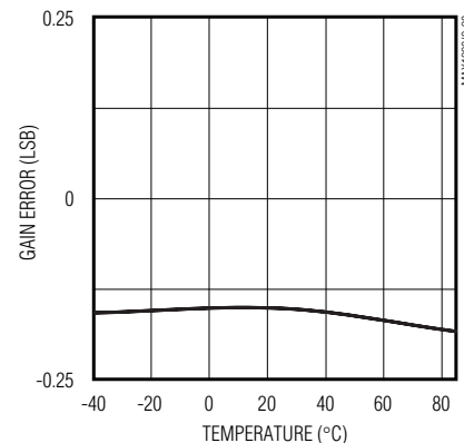
MAX1099 GAIN ERROR vs. TEMPERATURE
