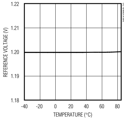
MAX1099 INTERNAL REFERENCE VOLTAGE vs. TEMPERATURE
