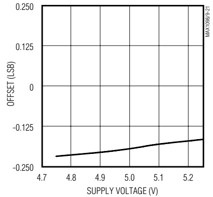
MAX1098 OFFSET vs. SUPPLY VOLTAGE
