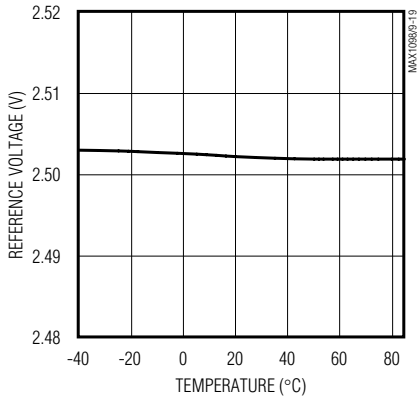
MAX1098 INTERNAL REFERENCE VOLTAGE vs. TEMPERATURE
