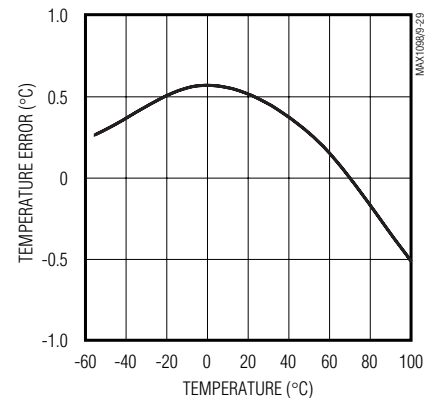
MAX1098 TEMPERATURE ERROR vs. INTERNAL DIODE TEMPERATURE
